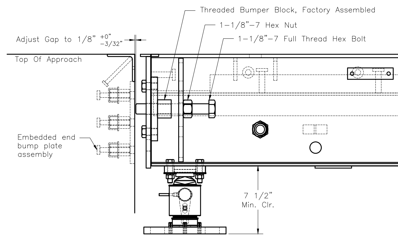
END CHECKING DETAIL Note: Side checking hardware not shown in this view for the sake of clarity
